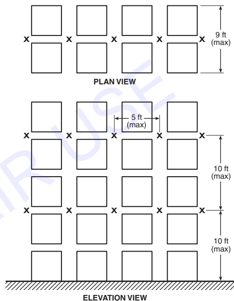
FIGURE 16.6.4(c) Double-Row Rack Sprinkler Layout I — Option #2.
