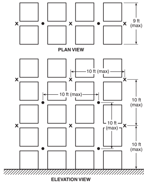
FIGURE 16.6.4(b) Double-Row Rack Sprinkler Layout I — Option #1.
