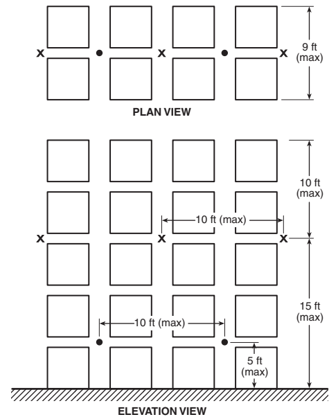
FIGURE 16.6.4(d) Double-Row Rack Sprinkler Layout H — Option #1.
