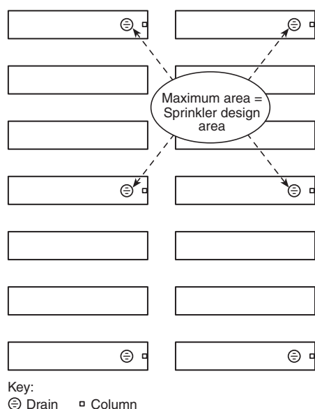
FIGURE A.16.8.2(d) Typical Arrangement of Floor Drains.
