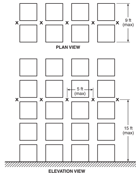
FIGURE 16.6.4(e) Double-Row Rack Sprinkler Layout H — Option #2.
