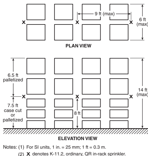
FIGURE 16.6.4(a) Double-Row Rack Sprinkler Layout G.
